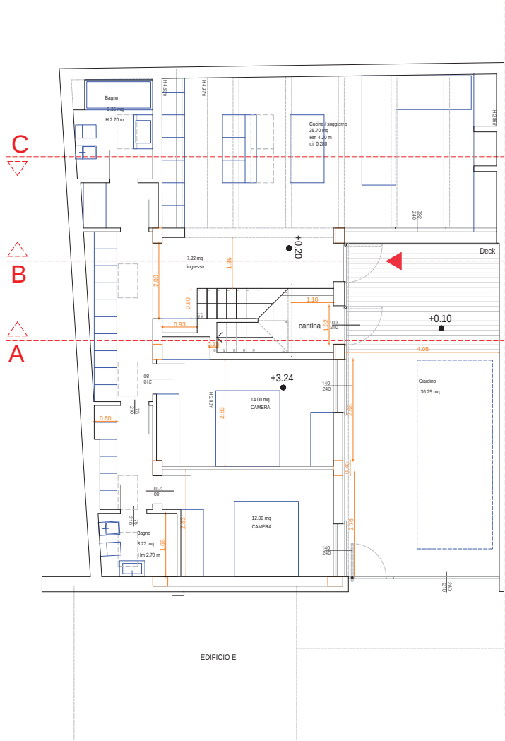
Piano terra
